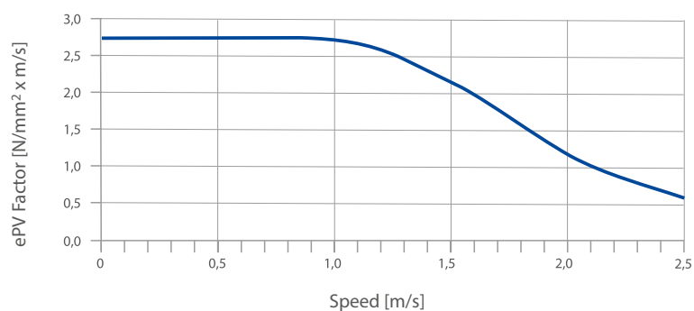
Fig. 11: Maximum ePV factor for grease lubrication
