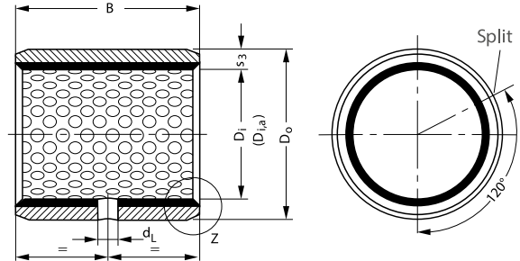
Dimensions and Tolerances according to ISO 3547 and GGB Specifications
