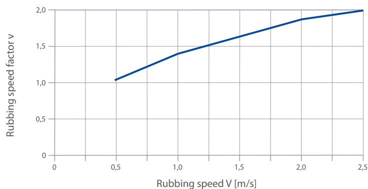
Fig. 22: Rubbing speed factor v
