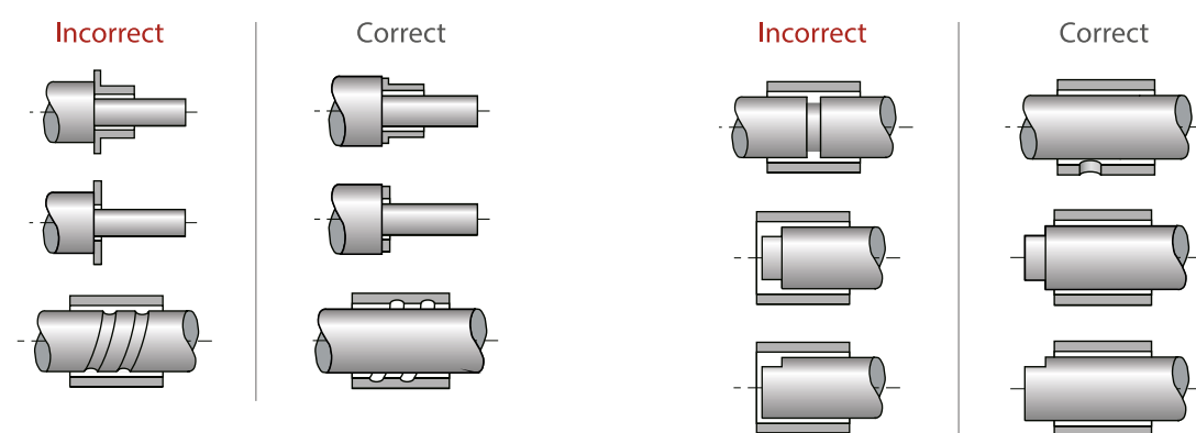
Fig. 25: Counterface Design
