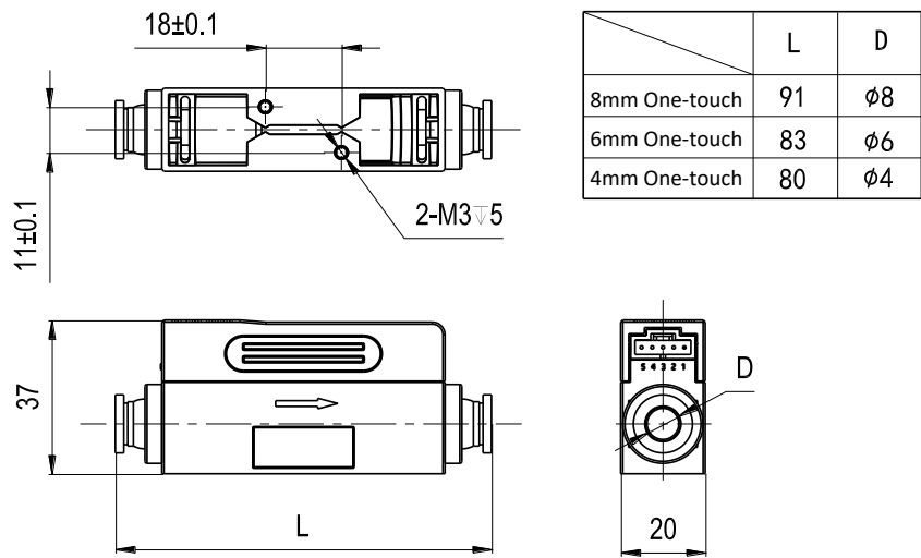
Figure 5: PFLOW3000 dimensions with one-touch connectors. All units are in mm
