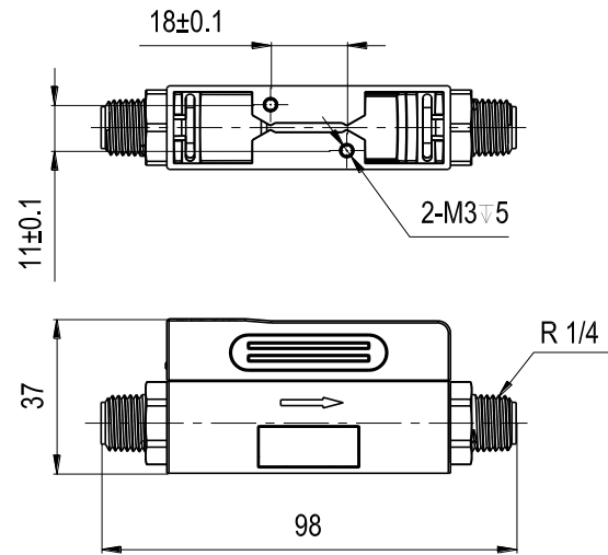
Figure 4: PFLOW3000 dimensions with BSPT (R1/4") connectors. All units are in mm
