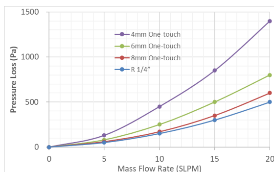
Figure 2: PFLOW3008-10/20SLPM pressure loss
