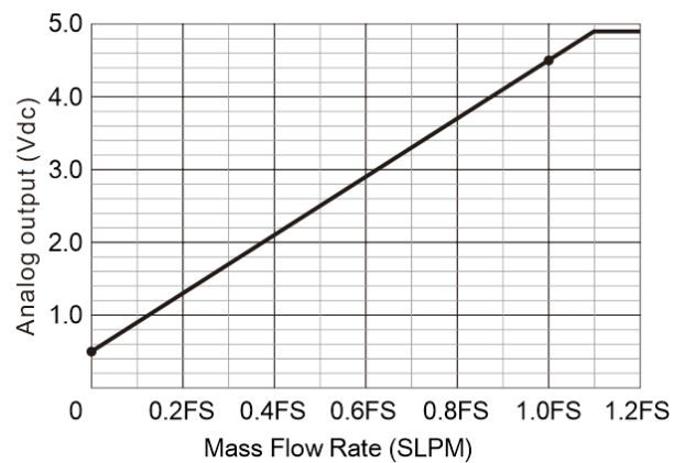
Figure 7: PFLOW3000 typical analog output
