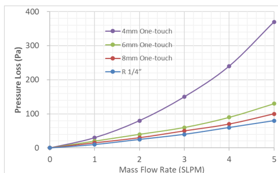
Figure 1: PFLOW3008-2/3/4/5SLPM pressure loss
