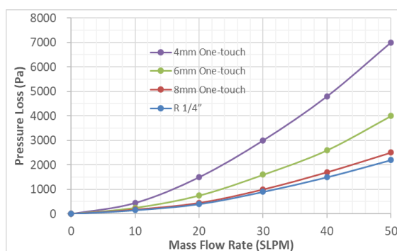
Figure 3: PFLOW3008-30/40/50 pressure loss
