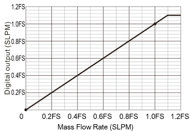
Figure 8: PFLOW3000 typical digital output
