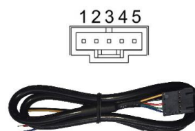
Figure 6: PFLOW3000 connection and cable
