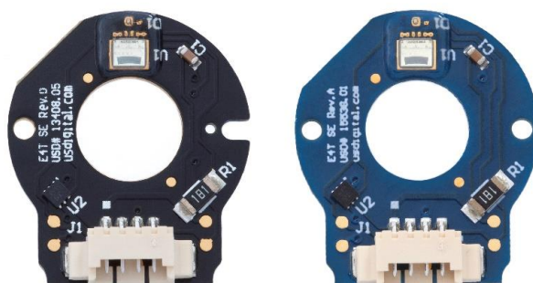
Figure 1, E4T PCB comparison showing existing design (left) vs. new board design (right).
