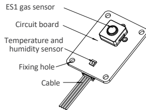
Product Schematic
