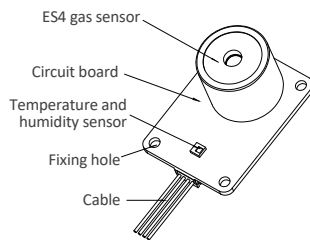
Product Schematic
