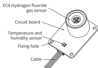
Product Schematic
