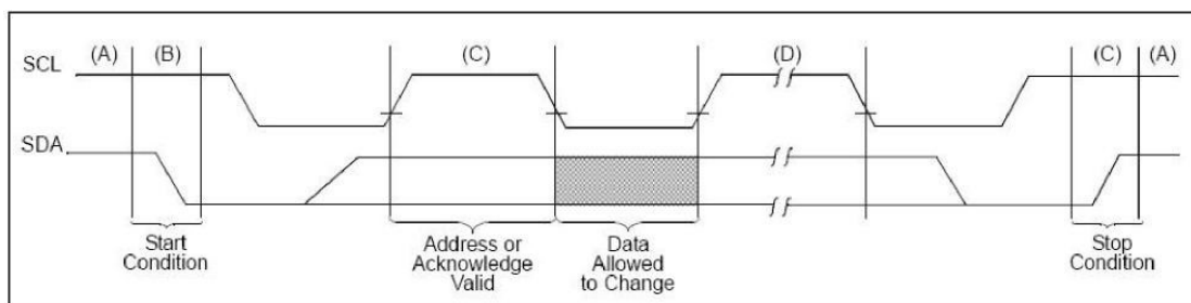
Fig. 3-1: Timing diagram of the I 2 C bus
