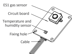
Product Schematic
