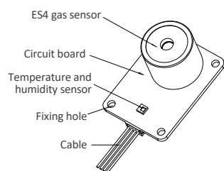
Product Schematic
