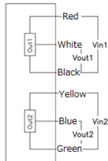
Dual Output, 6wires
