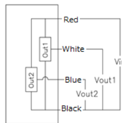
Dual Output, 4wires
