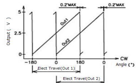
CP-45HP(180°Phase Output)
