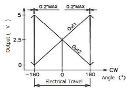
CP-45HP-5V Parallel Output
