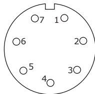
Binder 712 connector
