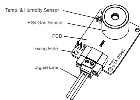
Product Schematic
