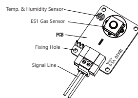
Product Schematic
