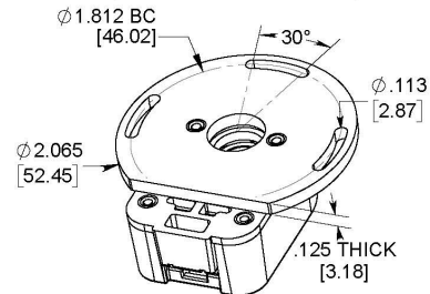
R-OPTION BASE (ROTATIONAL MOUNTING)
