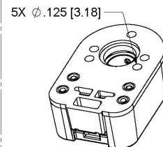
3-OPTION BASE (LARGER MOUNTING HOLES)
