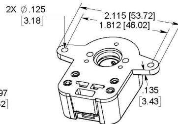
G-OPTION BASE (1.812" MOUNTING)
