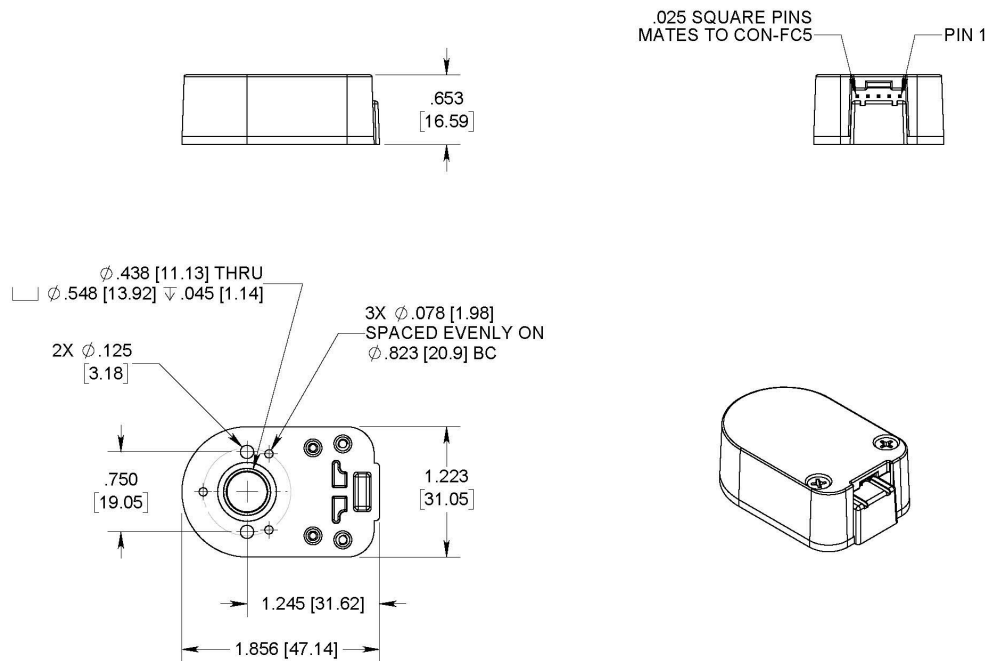
E5 Single-Ended Optical Kit Encoder (Default)
