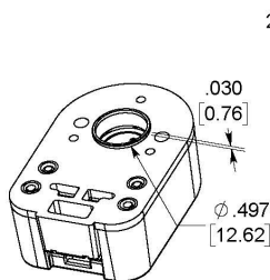
A-OPTION BASE (ALIGNMENT BOSS)
