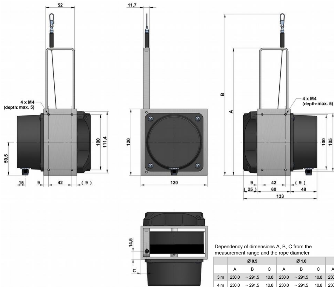
Standard: open housing + open rope bridge
