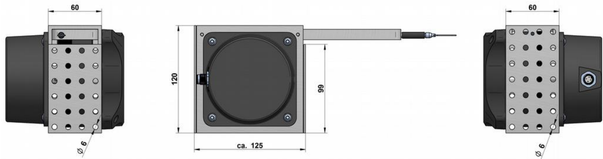
Version COV1: housing with perforated plate covering + open rope bridge
