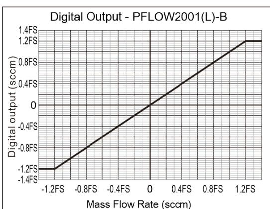
Figure 6: typical digital output curve of PFLOW2001(L)-B.
