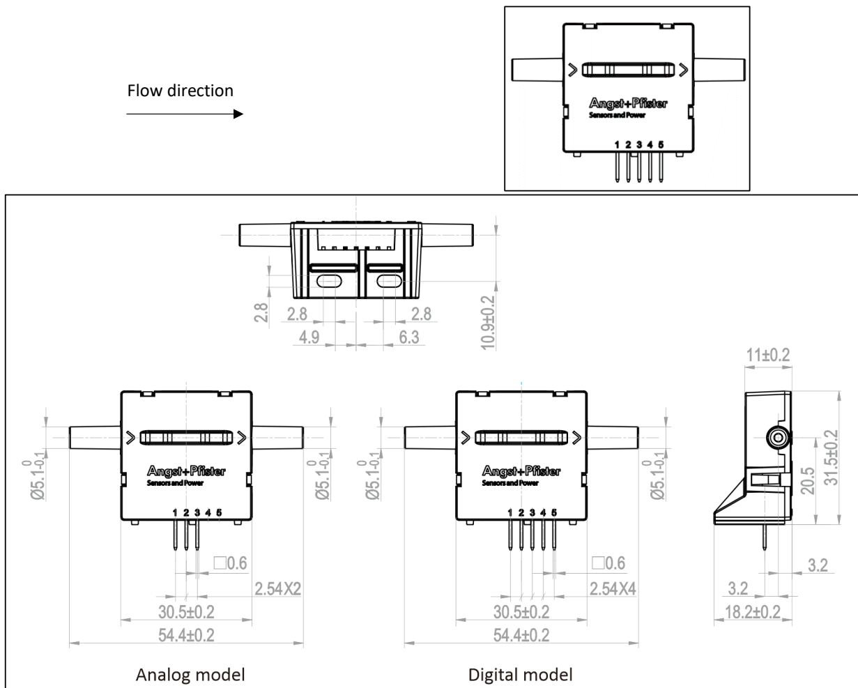
Figure 1 PFLOW2001. All units are in mm
