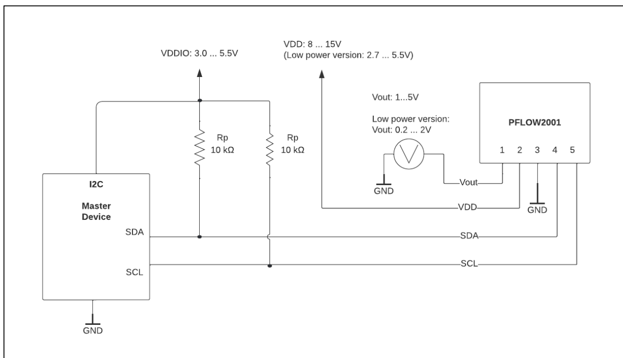
Figure 7. Analog and I2C interface connection diagram
