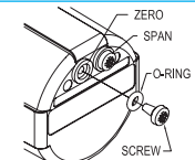
ZERO & SPAN ACCESS
