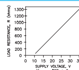
LOAD RESISTANCE VS INPUT VOLTAGE
