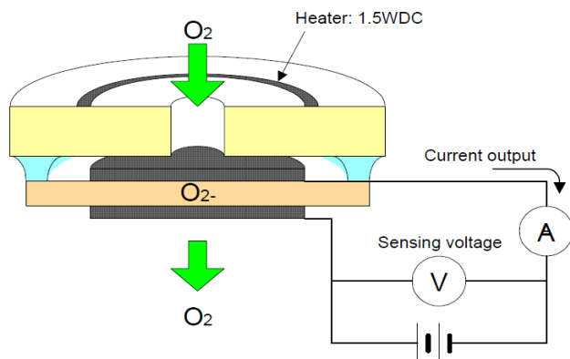
Fig. 1. Principle operation of the FCX oxygen sensor
