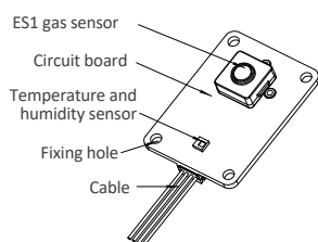
Product Schematic
