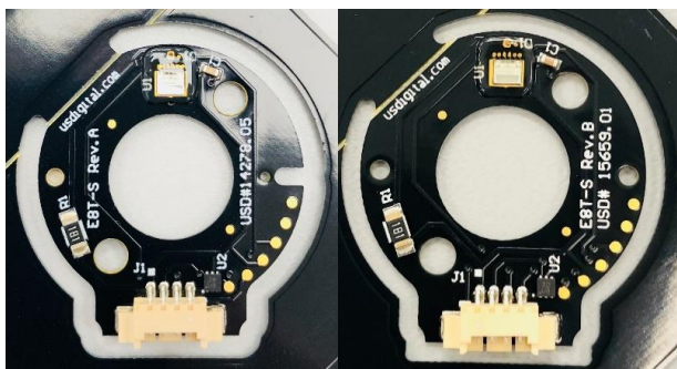
Figure 1, E8T PCB comparison showing existing design (left) vs. new board design (right).
