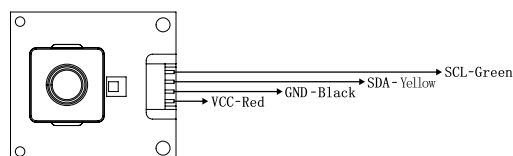
I 2 C 3.3V
