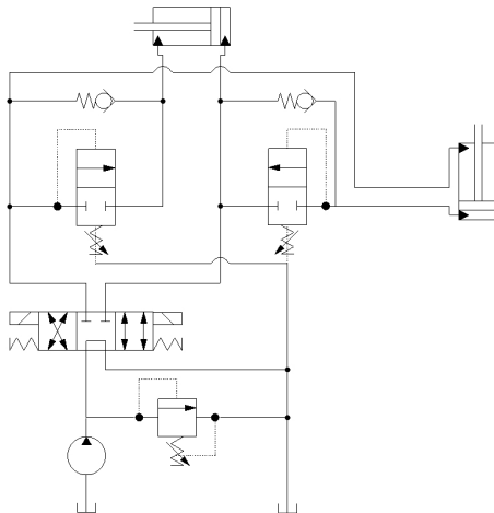
Sequencing Circuit
