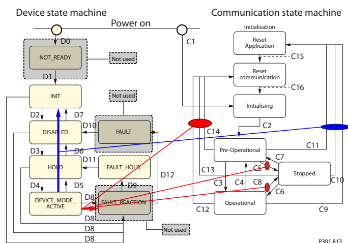
Device State Machine and Communication State Machine
