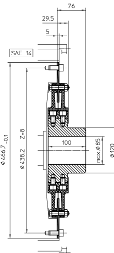
CF-K-200-D SAE 14
