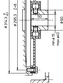
CF-K-100 SAE 10
