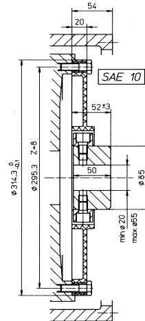
CF-K-125 SAE 10
