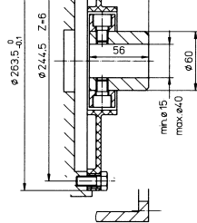
CF-K-100 SAE 8
