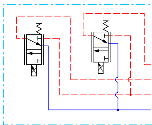
PVHC schematic
