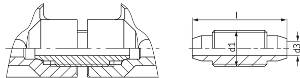
Distributor connection
