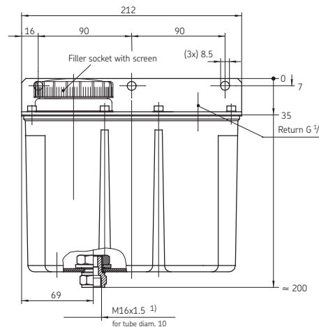
3-liter reservoir (shown: K3-S2)
