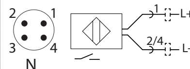
2-wire DC PNP/NPN
