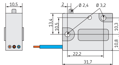
Electrical connection
