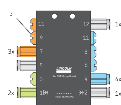
Fig. 18 Internal cross-porting
