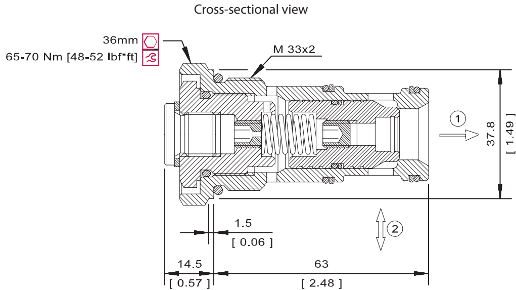
Check Valve
