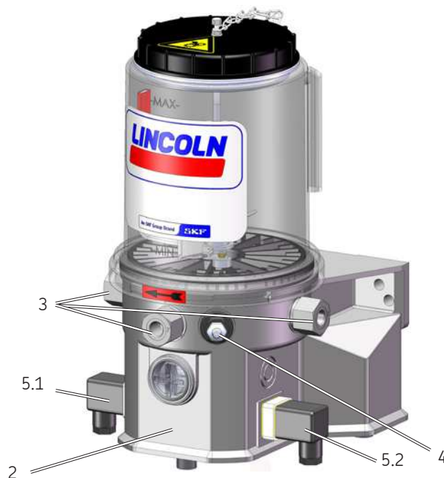
Overview, functional description of pumps without follower plate Fig. 2
