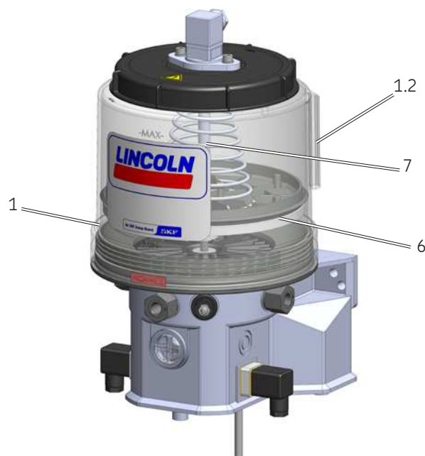
Overview, functional description of pumps with follower plate Fig. 3
