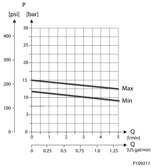
Accessory module for PVPV 256
