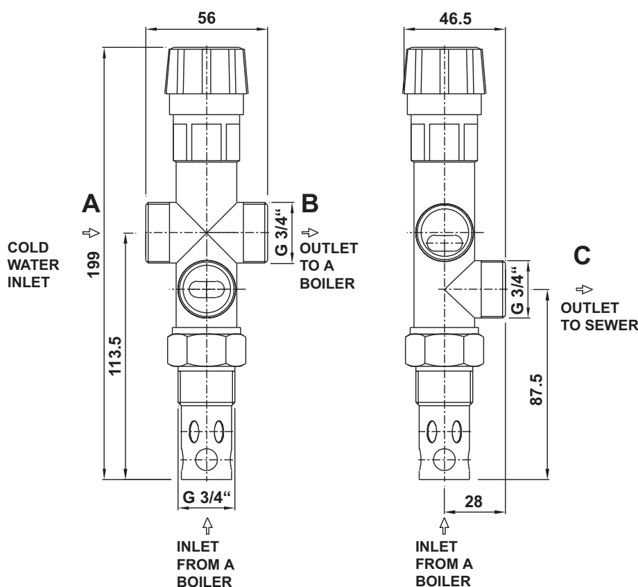
Pic. 1: Dimensional drawing
