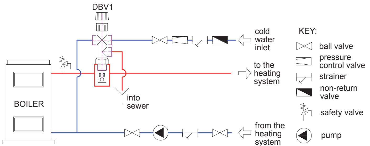
Pic. 3: Piping diagram for DBV1
